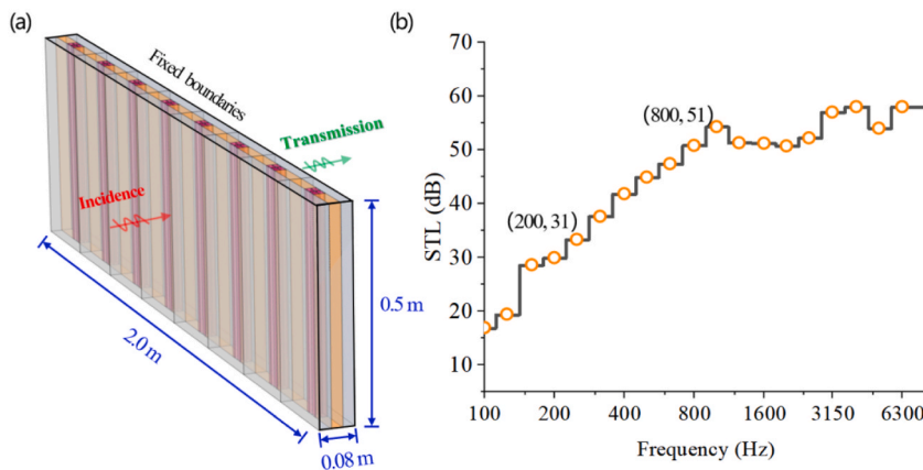
Fig. 8. Acoustic transmission loss. (a) Schematic of the simulation model. (b) STL.
